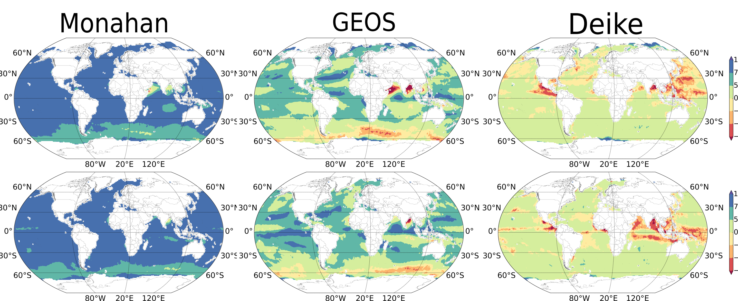
Fig 3. Seasonal Normalized Mean Difference : (Observed – Predicted)/(observed)WC fraction June-August(top), April-May (bottom)
