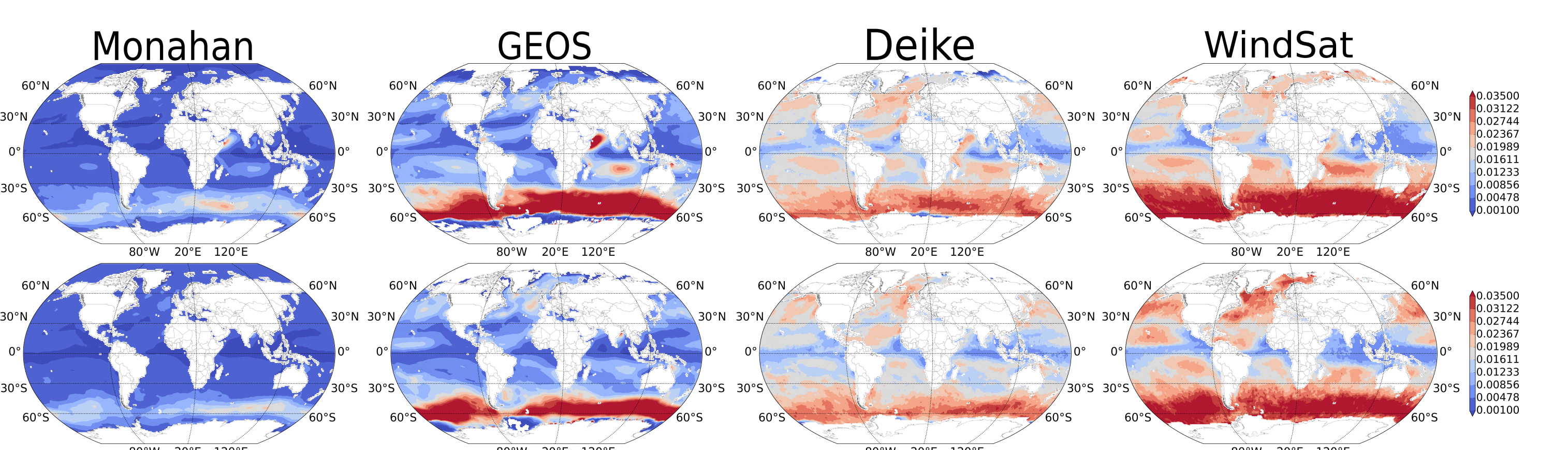
Fig 2. Seasonal means WC fraction June-August(top), April-May (bottom)
