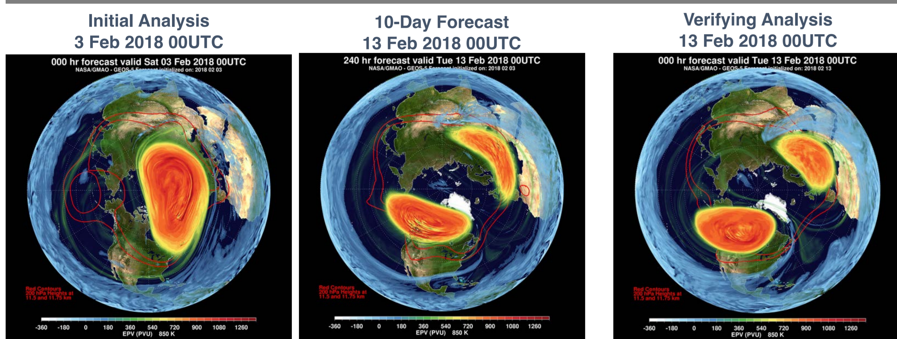
EPV on the 850 K Potential Temperature Surface (~30 km)
