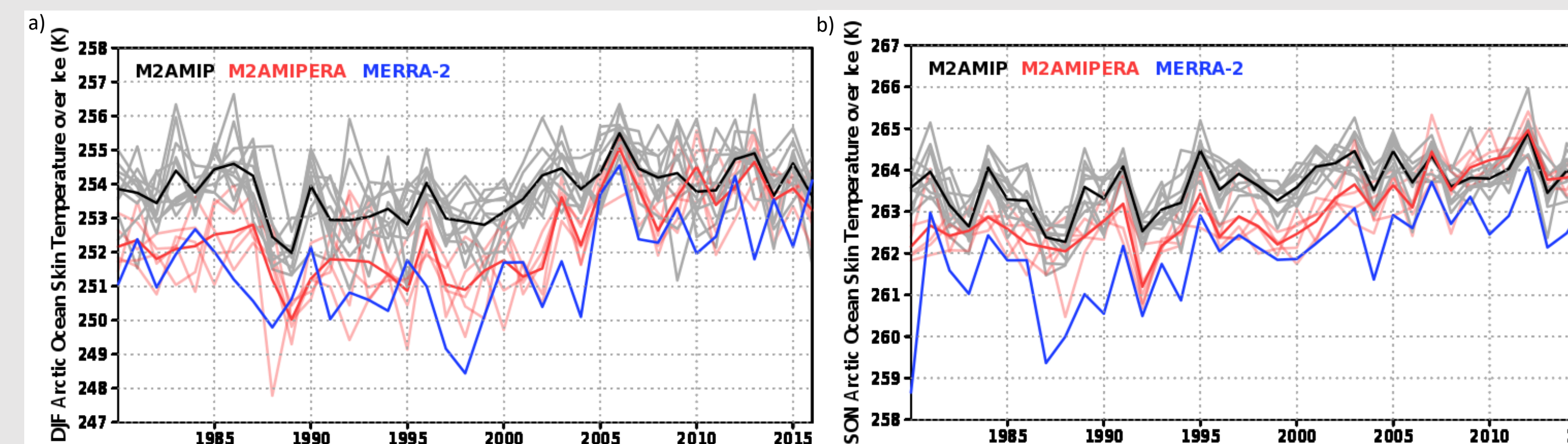
Figure 4: Seasonal mean skin temperature over ice in the Arctic Ocean in MERRA-2, M2AMIP, and M2AMIPERA during a) December-January-February and b) September-October-November
