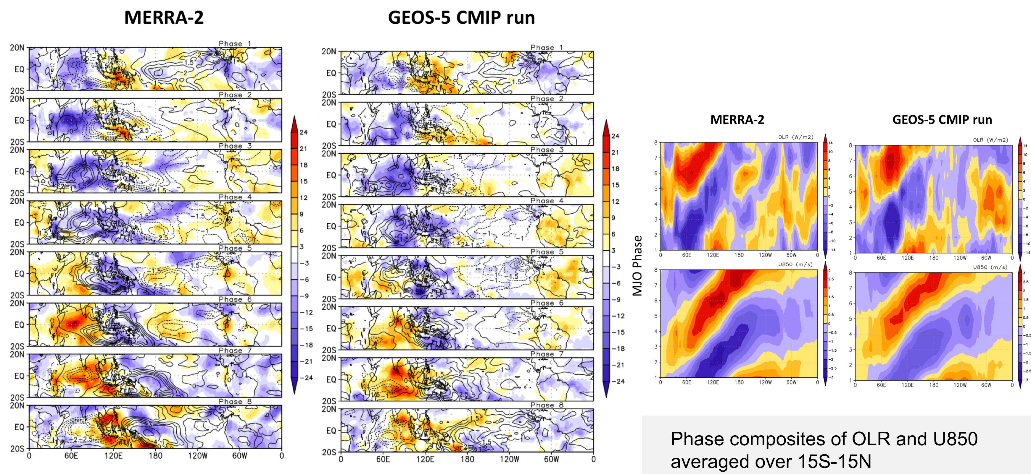
MJO RMM phase composites of OLR (shaded, W m^{-2} ) and U850 ( m s^{-1} ) in MERRA-2 and free running GEOS-5, the version employed in the SubX reforecasts
