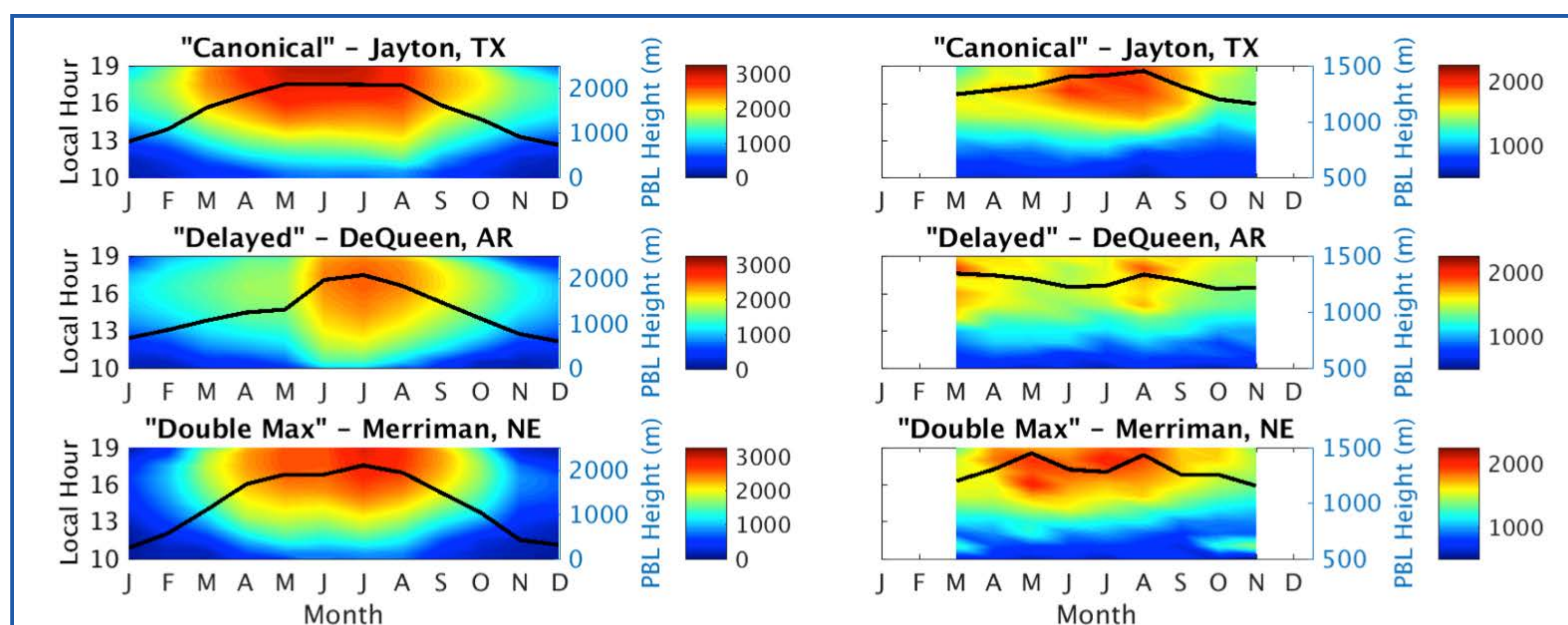
Figure 5: Monthly mean annual and diurnal cycle of PBL height in (left) MERRA-2 and (right) from WP at stations representing the three classes of behavior for the US Great Plains region: "canonical", "delayed", and "double maxima".
