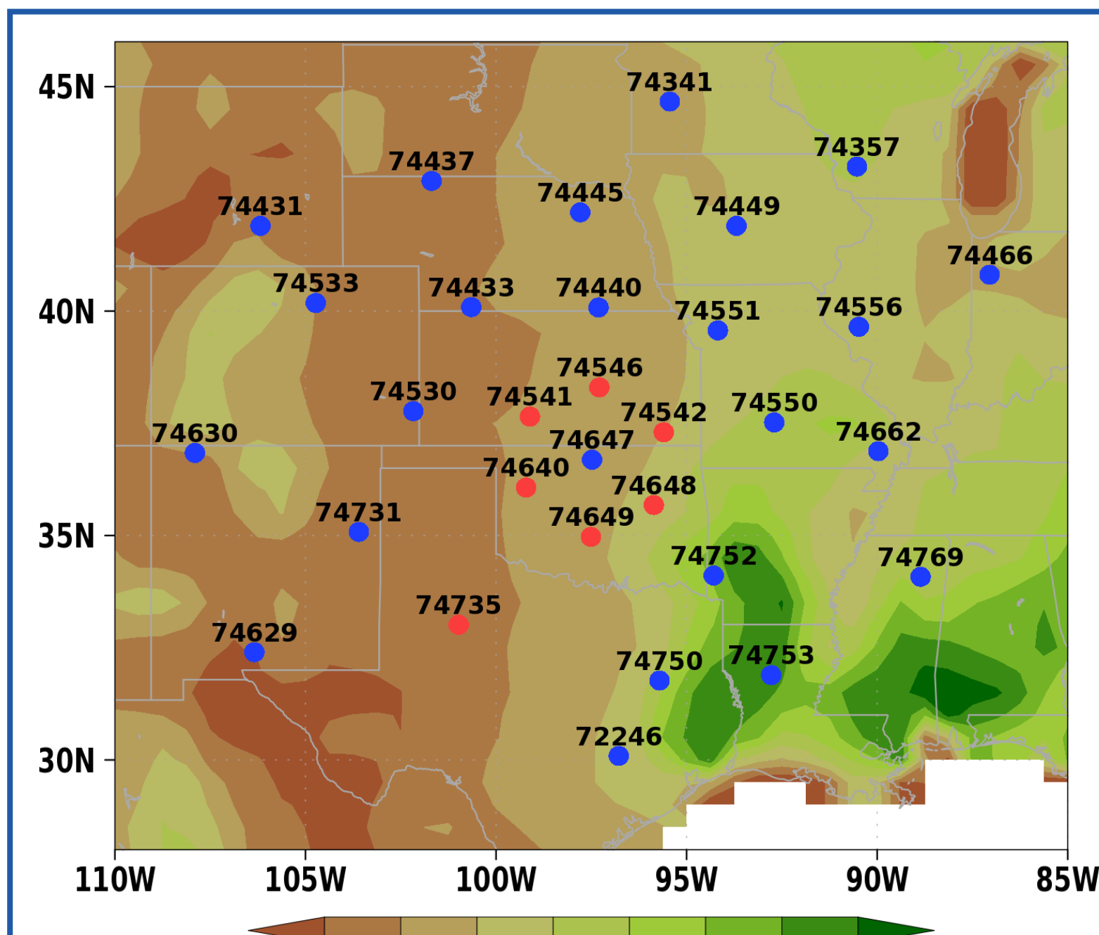
Figure 1: MERRA-2 LAI averaged over 1992-2012 overlaid with the location of WP stations used here.
