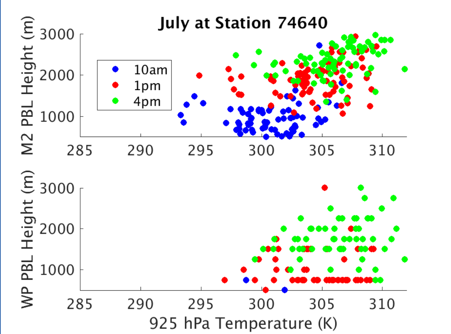
Figure 2: MERRA-2 and WP PBL height versus MERRA-2 925 hPa temperature Agreement in the relationship of PBL height to 925 hPa T gives confidence in the use of MERRA-2 for explaining the behavior of WP PBL height
