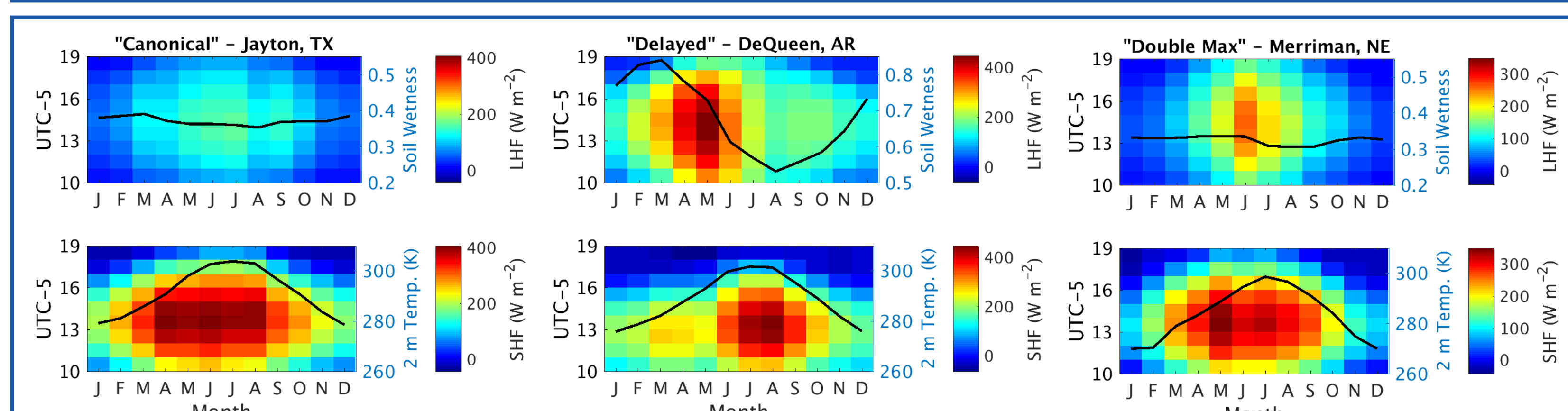
Figure 6: Monthly mean annual and diurnal cycle of (top row) latent heat flux, overlaid with root zone soil moisture and (bottom row) sensible heat flux overlaid with 2 m temperature at the three representative stations in Figure 5.
