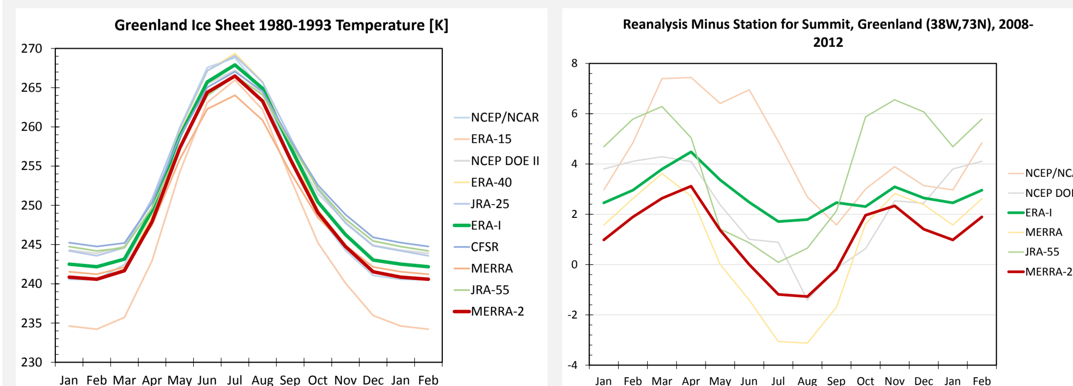
Figure 4. Average annual cycle for (left) 1980-1993 for the full GrIS, and (right) differences with Summit Station, 2008-2012.
