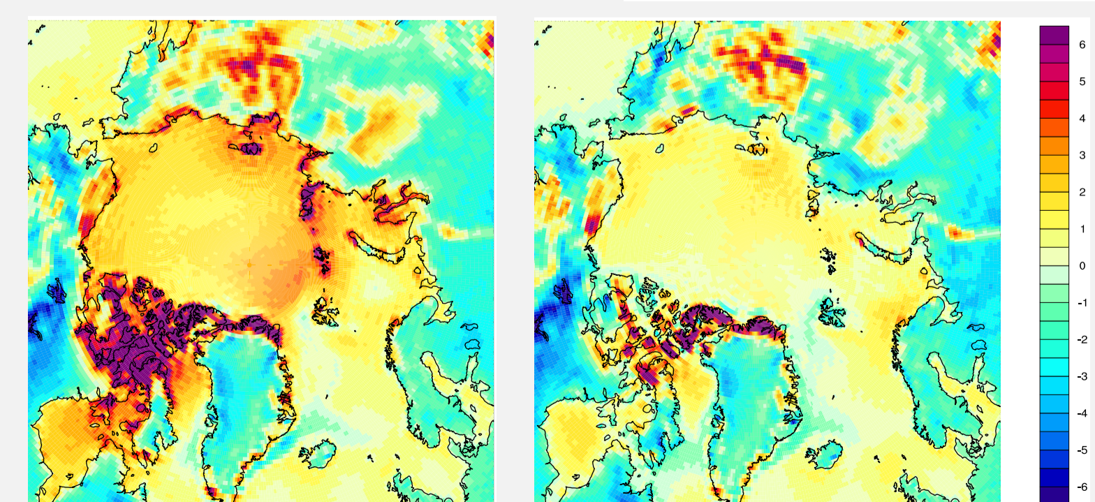
Figure 7. MERRA-2 Minus ERA-I temperature for DJF (left) 1980-2004, and (right) 2010-2016. In the latter period, both reanalyses used the same boundary data.
