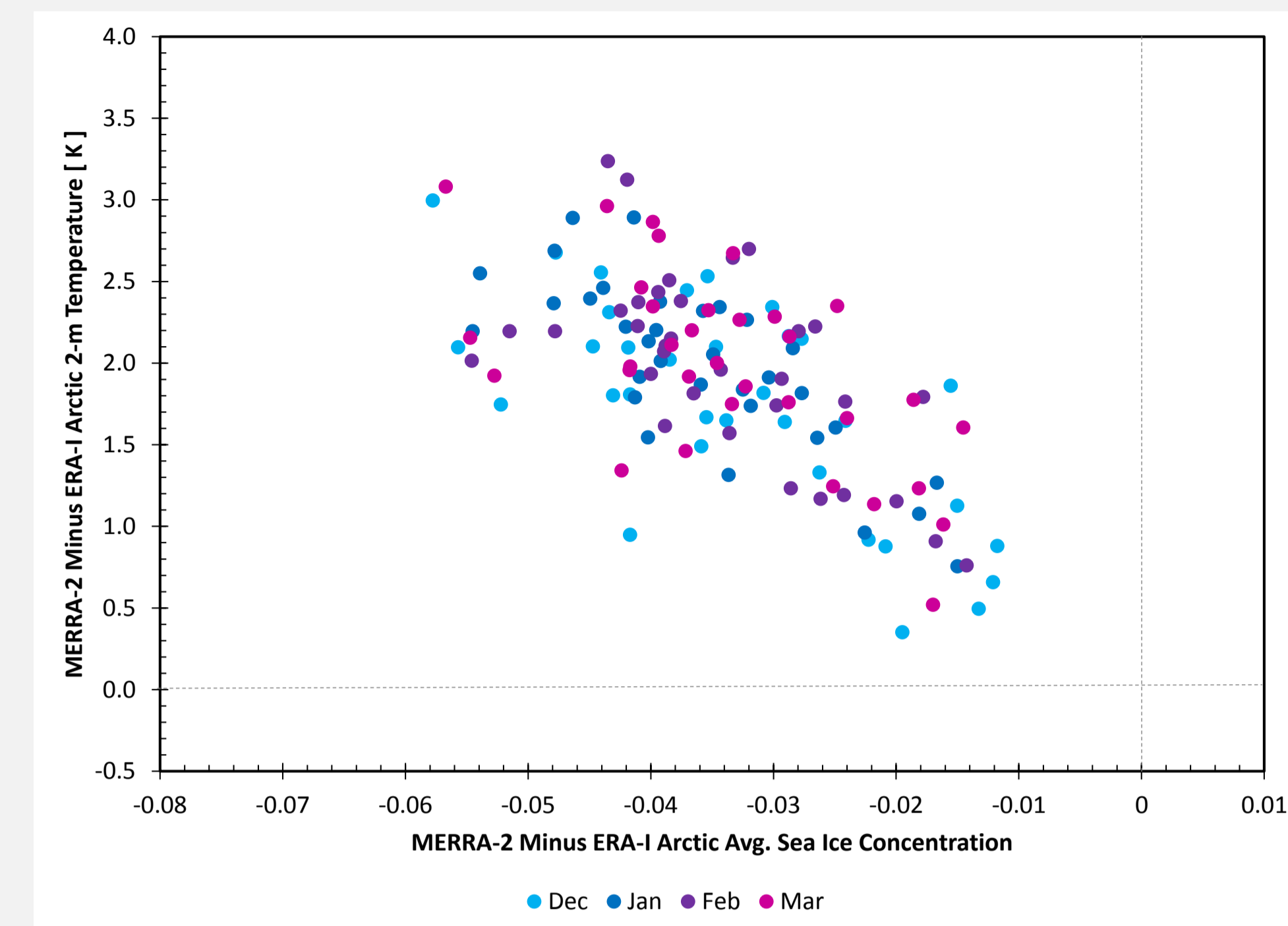
Figure 8. Scatter of MERRA-2 minus ERA-I temperature, versus MERRA-2 minus ERA-I sea ice concentration. Each point indicates an average over the central Arctic Ocean for an individual month.
