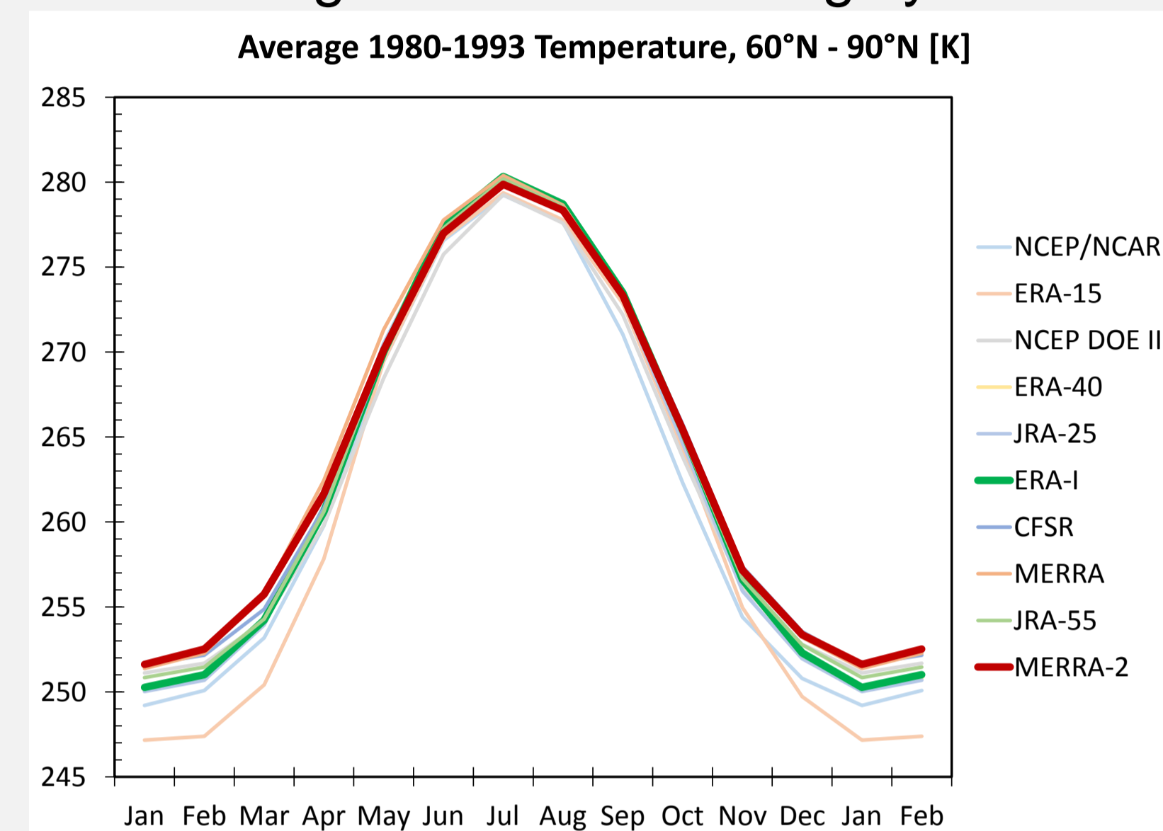
Figure 3. Average annual cycle for the north polar cap (60°N - 90°N) for common period 1980-1993.
