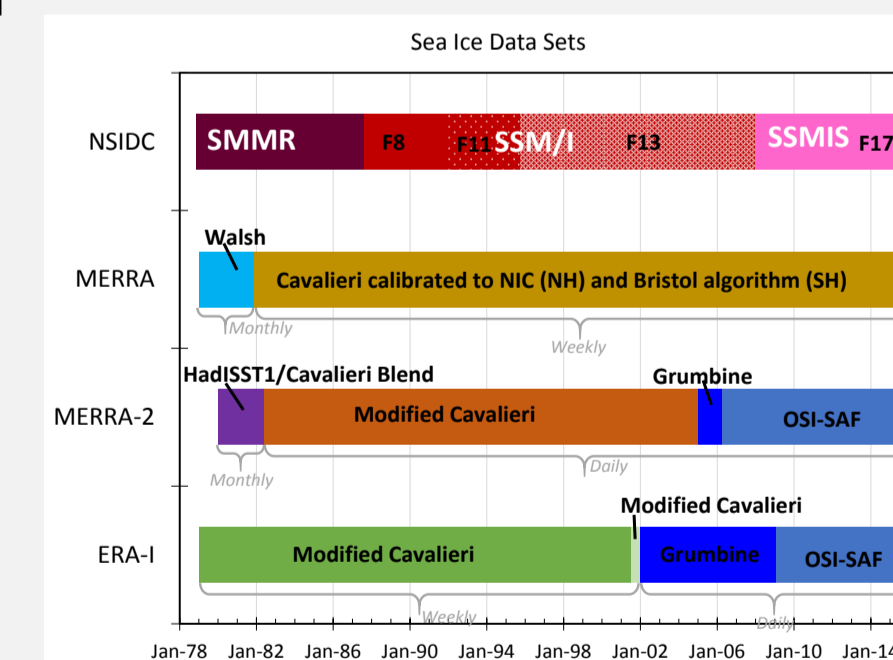
Figure 6. Time series of sea ice data sets used in reanalyses.
