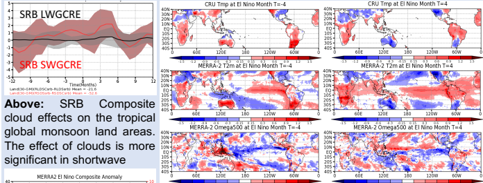
Above: SRB Composite cloud effects on the tropical global monsoon land areas. The effect of clouds is more significant in shortwave
