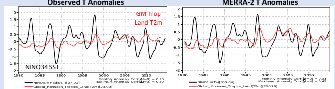
Above: De-seasonalized detrended temperature anomalies for Niño34 and Global Monsoon Land regions in observations and MERRA-2, showing lag of the land warming behind the SST warming.
