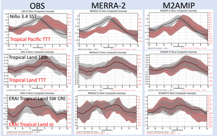
Above: Composite area average time series of Observations (left) MERRA-2 (center) M2AMIP (right) for Niño 3.4 surface temperature and near surface air temperature (top), Tropical land T2m and TTT (middle), SWCRE and pressure velocity (bottom). The time series of monthly means have been deseasonalized and detrended. Shaded areas represent +/-1 standard deviation. Here, Tropics are bounded by 30S-30N, and the land regions are within the defined Global Monsoon area. ERA-Interim (Dee et al. 2011) replaces observations in the lower left as a point of comparison.
