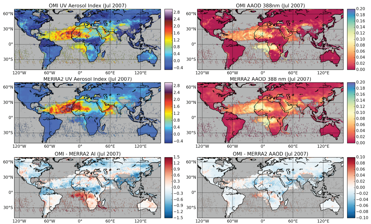
Figure 4.6: Monthly mean UV AI (left column) and AAOD (right column) at 388 nm from OMI (top row) and simulated from MERRA-2 (middle row) in July 2007. Difference plots (OMI - MERRA-2) are on the bottom row. MERRA-2 AI is simulated as described in Buchard et al. (2015) .
