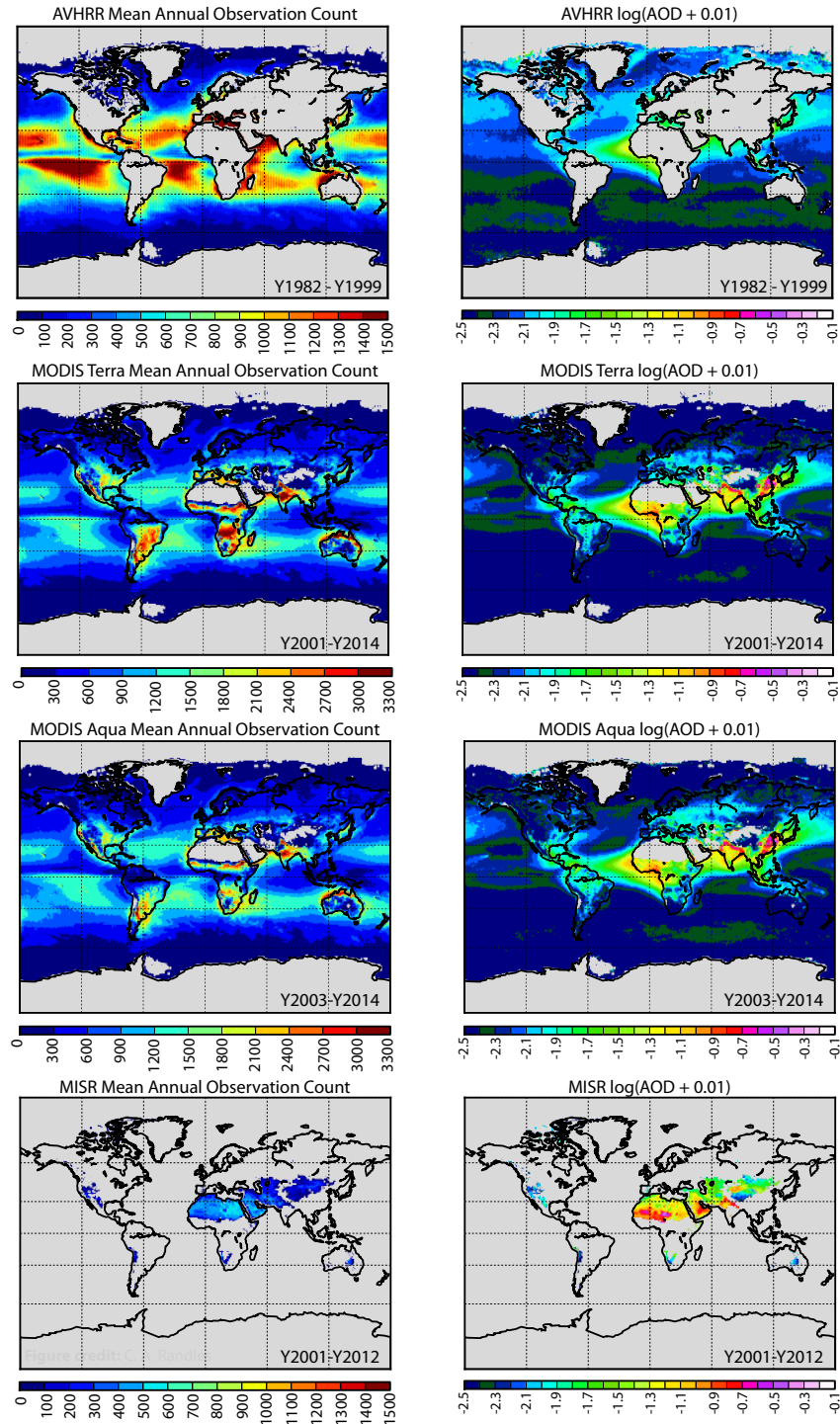
Figure 3.2: Climatological annual-mean number of observations (left) and annual mean \log(AOD + 0.01) (right) included in the assimilation from AVHRR (top row 1982-1999), MODIS Terra (second row; 2001-2014), MODIS Aqua (third row; 2003-2014), and MISR (bottom row; bright surface only; 2001-2012). Grey shading indicates regions with no data. Note the different scales for the observation counts.
