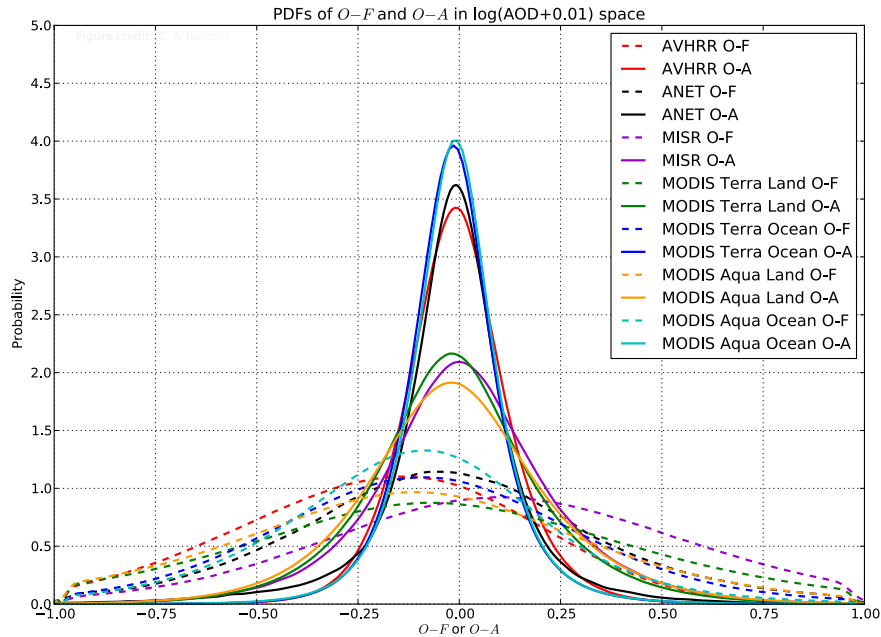
Figure 3.10: Probability distribution functions of all O - F (dashed lines) and O - A (solid lines) for AVHRR, MODIS, MISR, and AERONET (ANET). PDFs are for the time periods listed for each sensor in Table 3.2.
