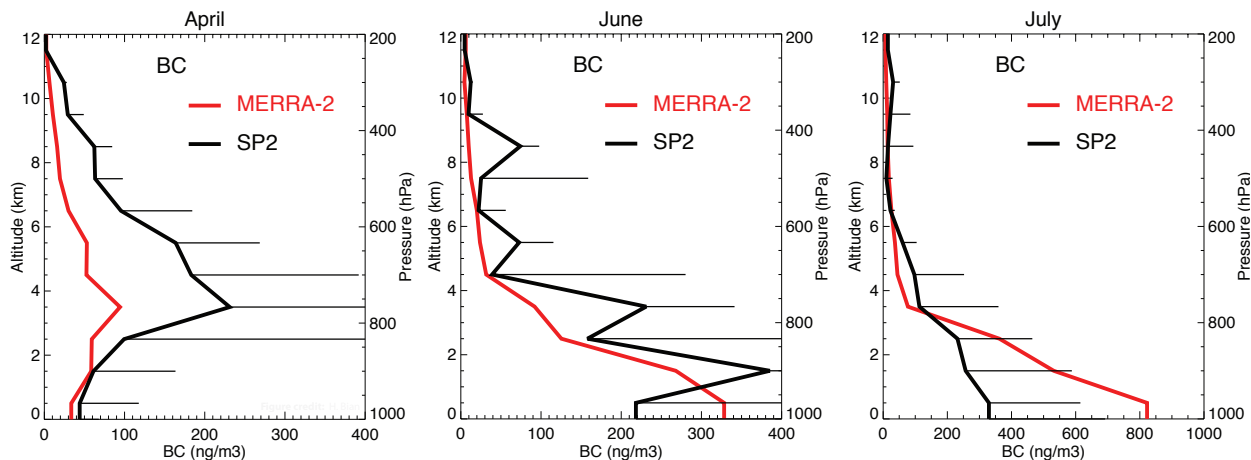
Figure 4.11: Comparison of MERRA-2 black carbon mass concentration [ \text{ng m}^{-3} ] to observations from the SP2 instrument during the (a) ARCTAS-A campaign (Fairbanks, Alaska; 3-19 April 2008), (b) the ARCTAS-CARB campaign (Palmdale, CA; 18-24 June, 2008), and (c) the ARCTAS-B campaign (Cold Lake, Alberta, Canada; 29 June -13 July, 2008).
