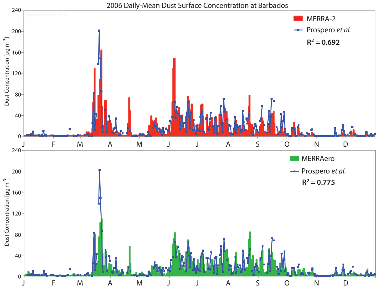
Figure 4.15: Daily-mean dust surface concentration [ \mu\text{g m}^{-3} ] at the RSMAS Barbados station [ 13.17^\circ\text{N} , 59.53^\circ\text{W} ] for 2006 compared to MERRA-2 (top) and MERRAero (bottom).
